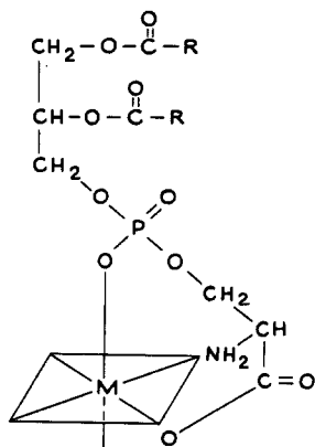
FIGURE 8: Possible structure for phosphatidylserine metal complex.
