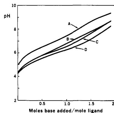
FIGURE 5: Titration curves for triphosphoinositide. A, Free ligand; B, Mg(II)-ligand (1:1); C, Ca(II)-ligand (1:1); D, Ni(II)-ligand (1:1) ( C_0 = 8.26 \times 10^{-4} M, \mu = 0.1 M).
